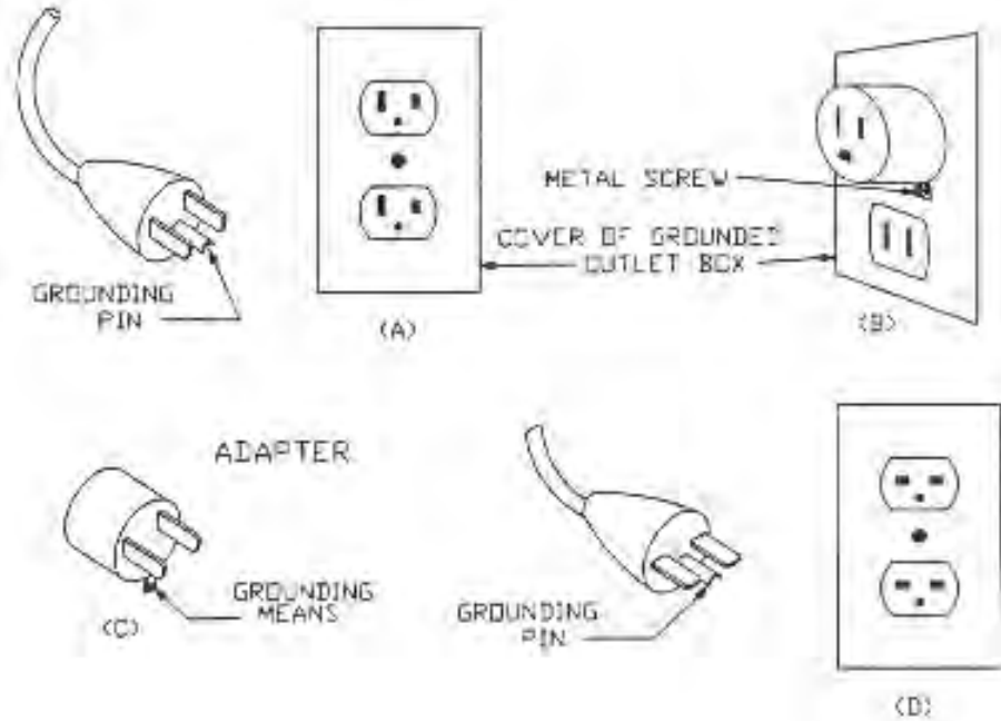
Fig. 1: Grounding Methods
